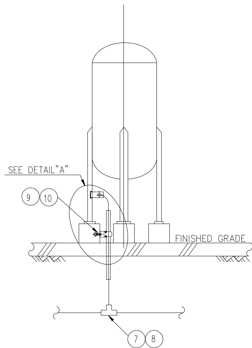
VERTICAL DRUM
