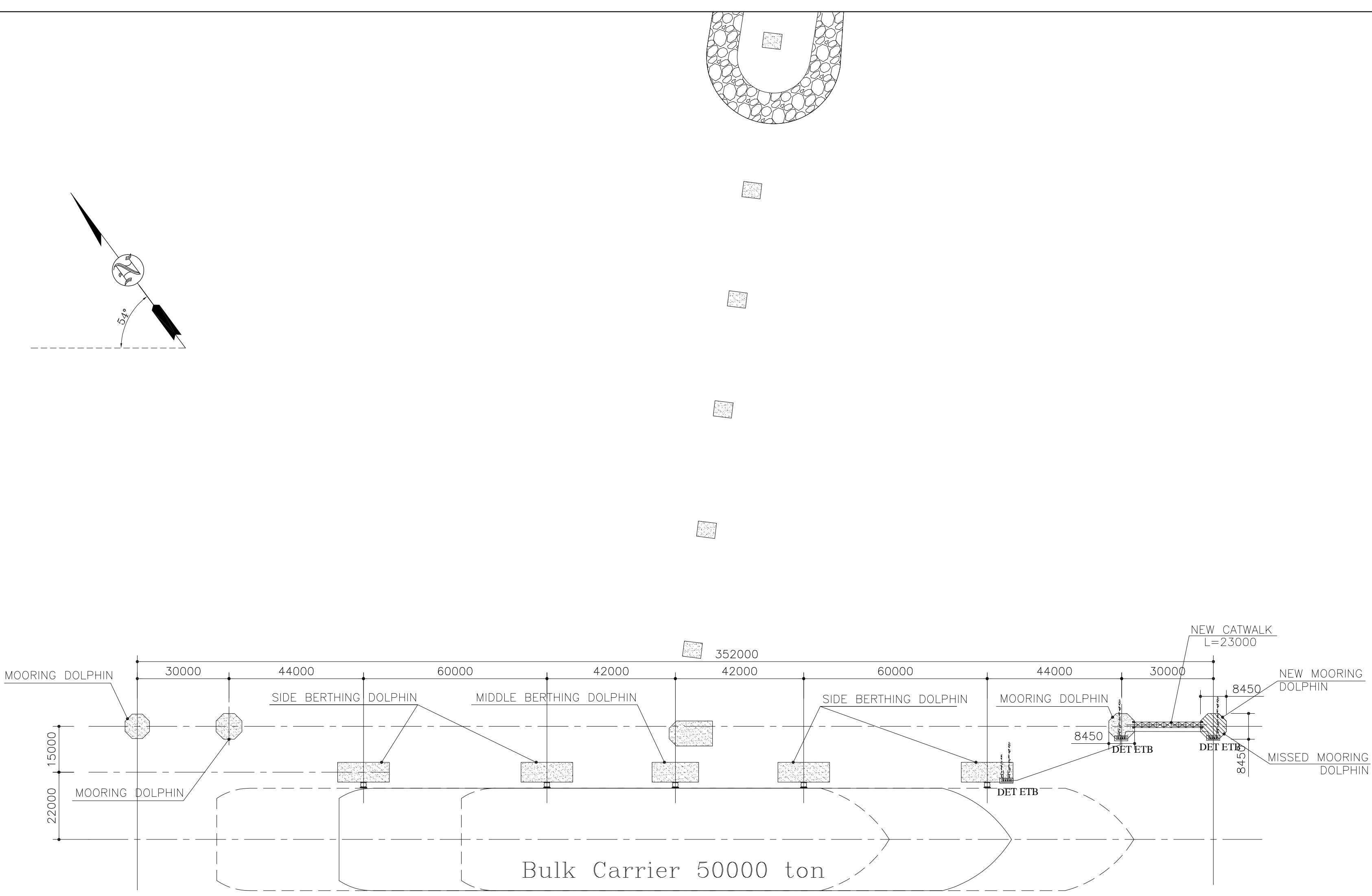
EARTHING LAYOUT- GENERAL LAYOUT OF JETTY SC.1:100
