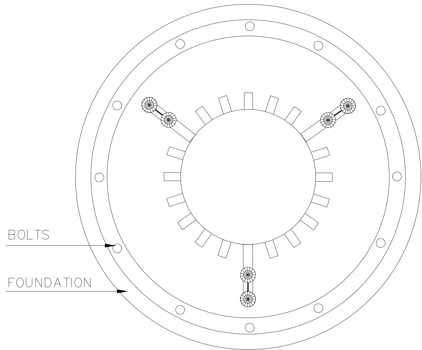
TOP VIEW
