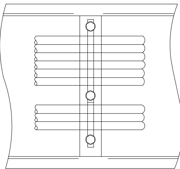
3) HORIZONTALY TRAY MOUNTED. HORIZONTAL CABLE RUN
