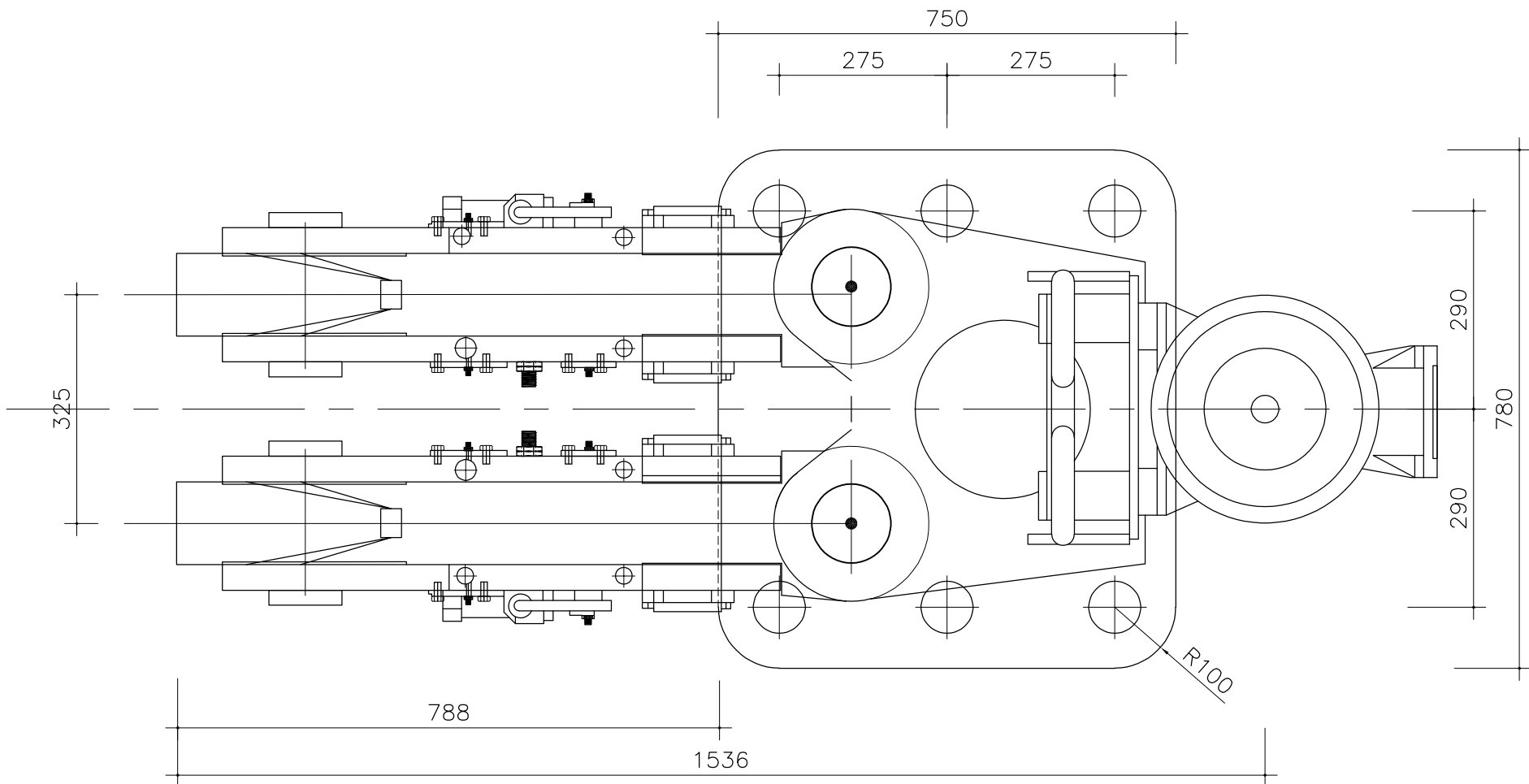
QUICK RELEASE 60-TON(DOUBLE HOOKS) N.T.S
