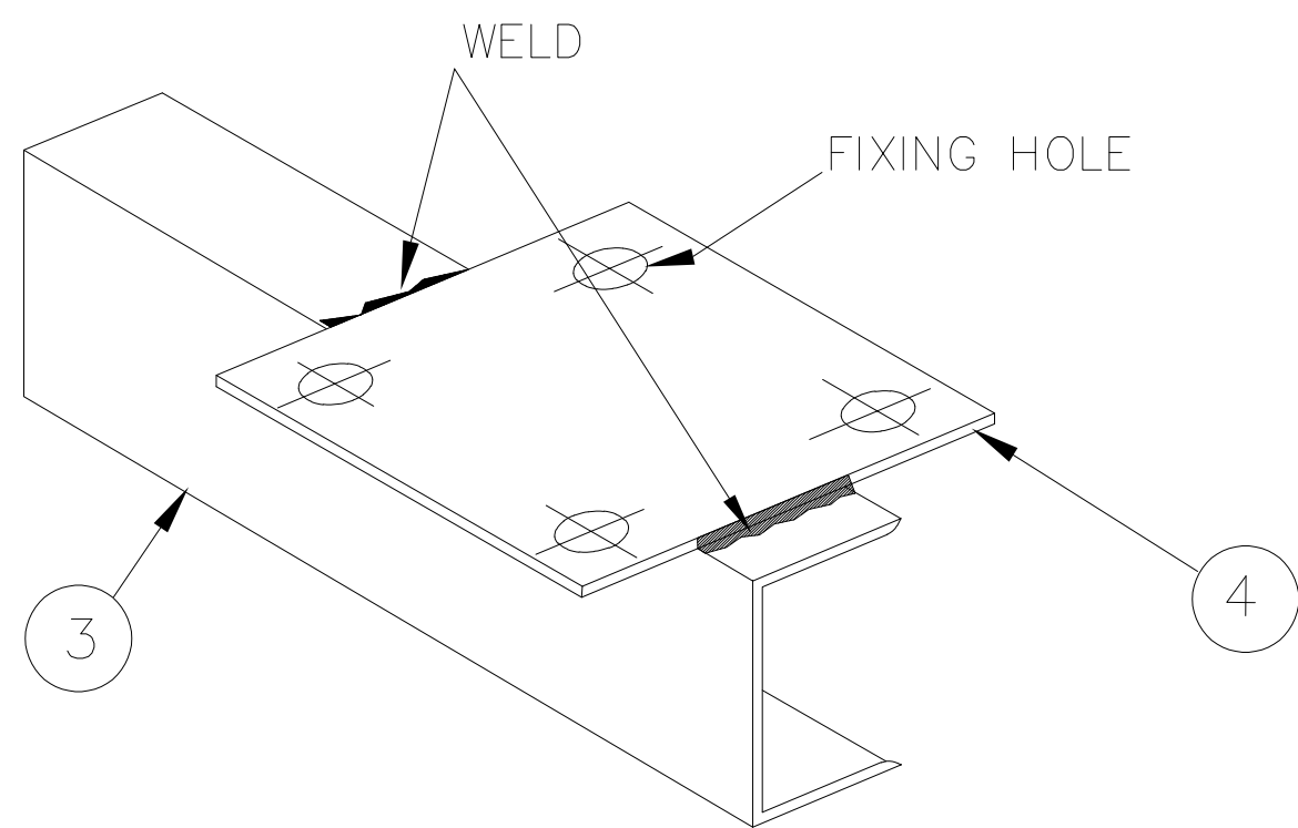
FIXTURE SUPPORT DETAIL
