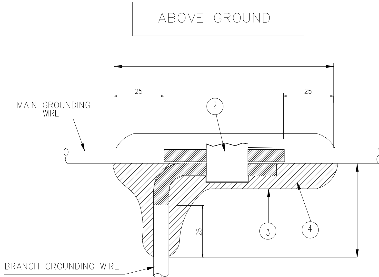
PARALLEL CONNECTOR
