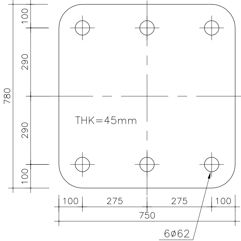
PLATE "A" SC.1:10
