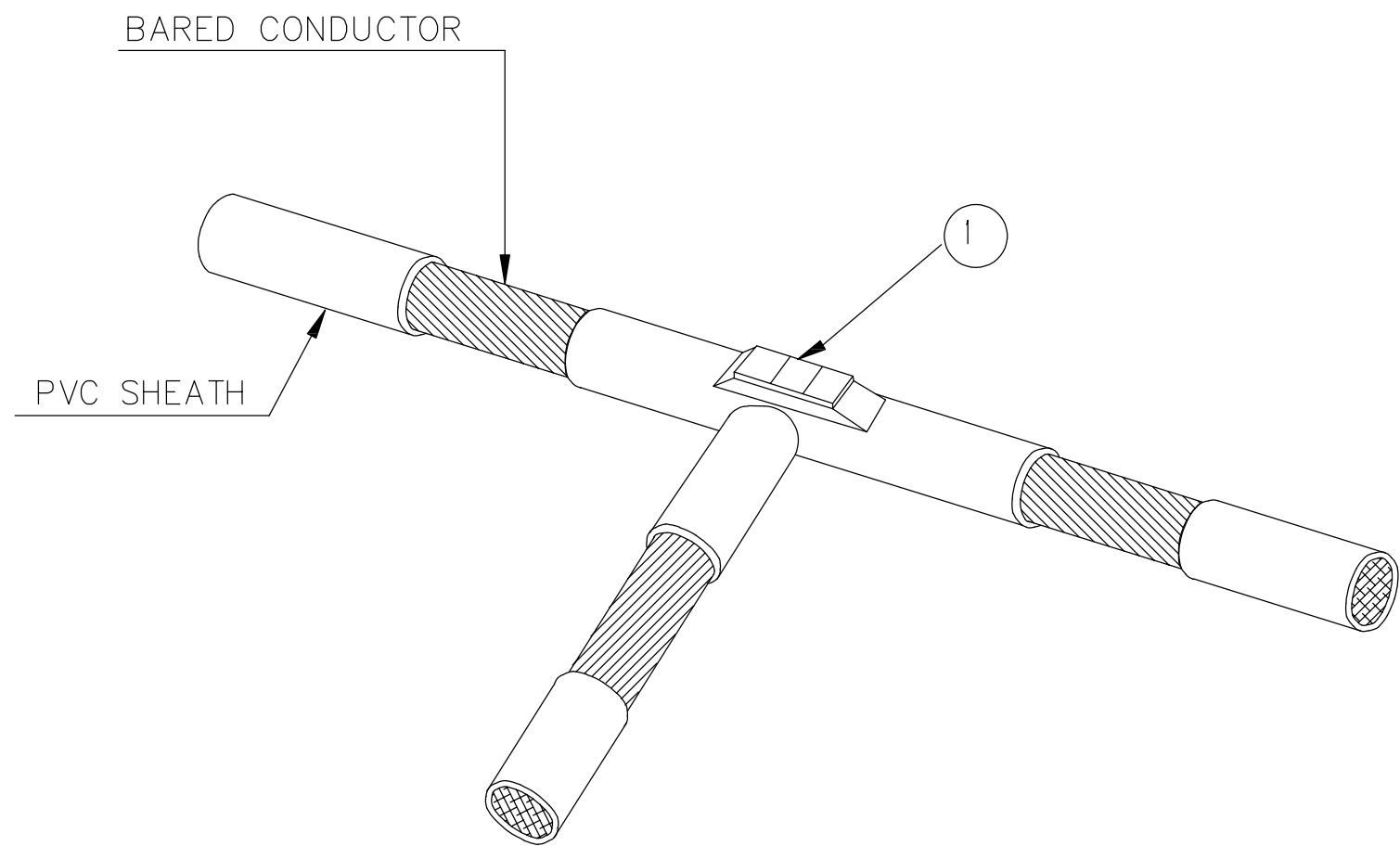
STRAIGHT JOINT
