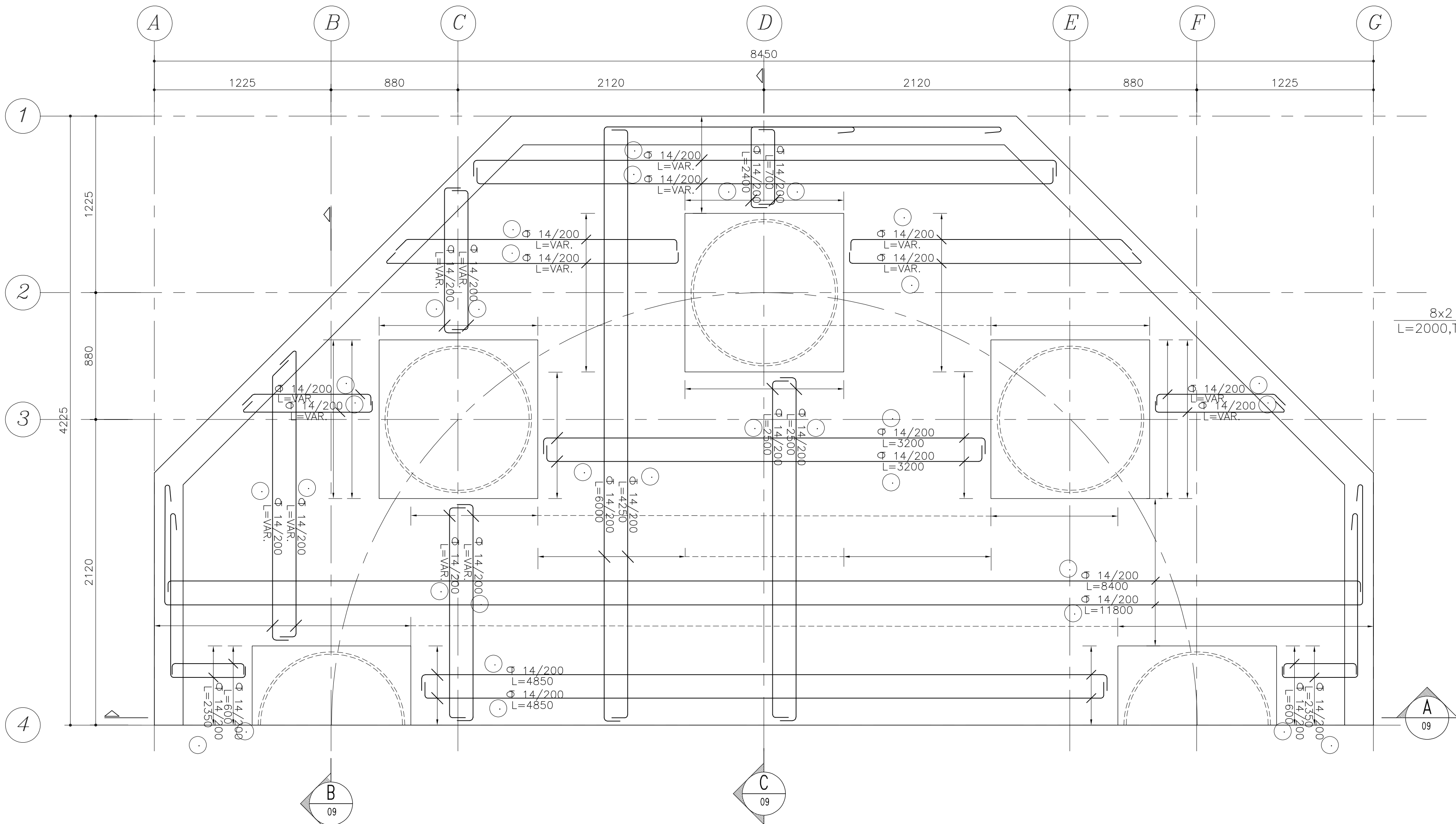
REINFORCEMENT CAISSON PLAN TYPE "1" SC.1:20
