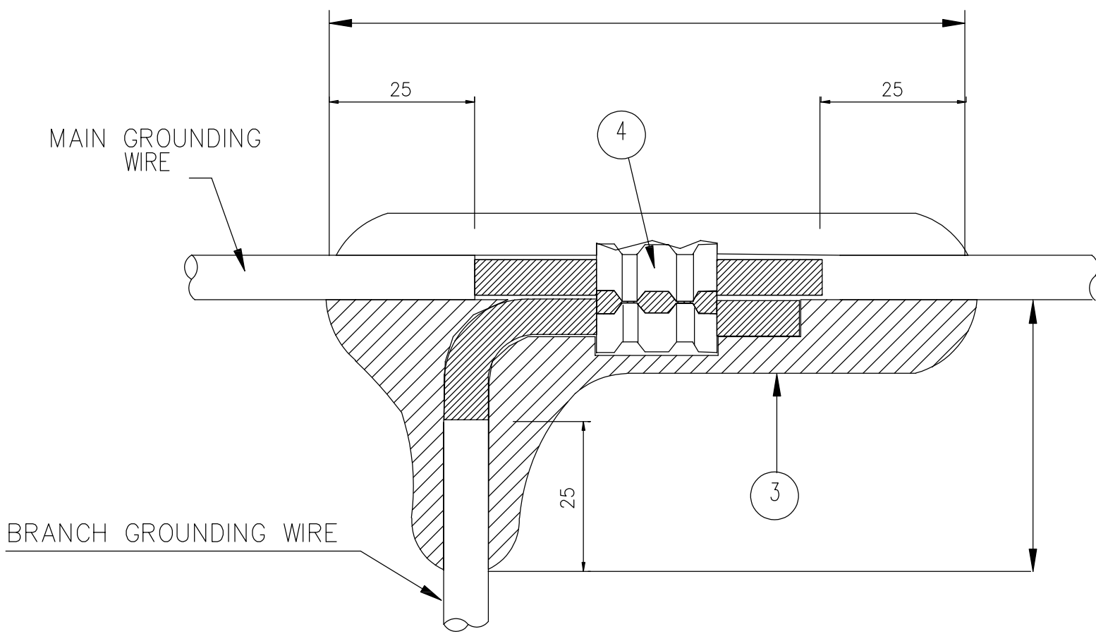
"C" TYPE CONNECTOR
