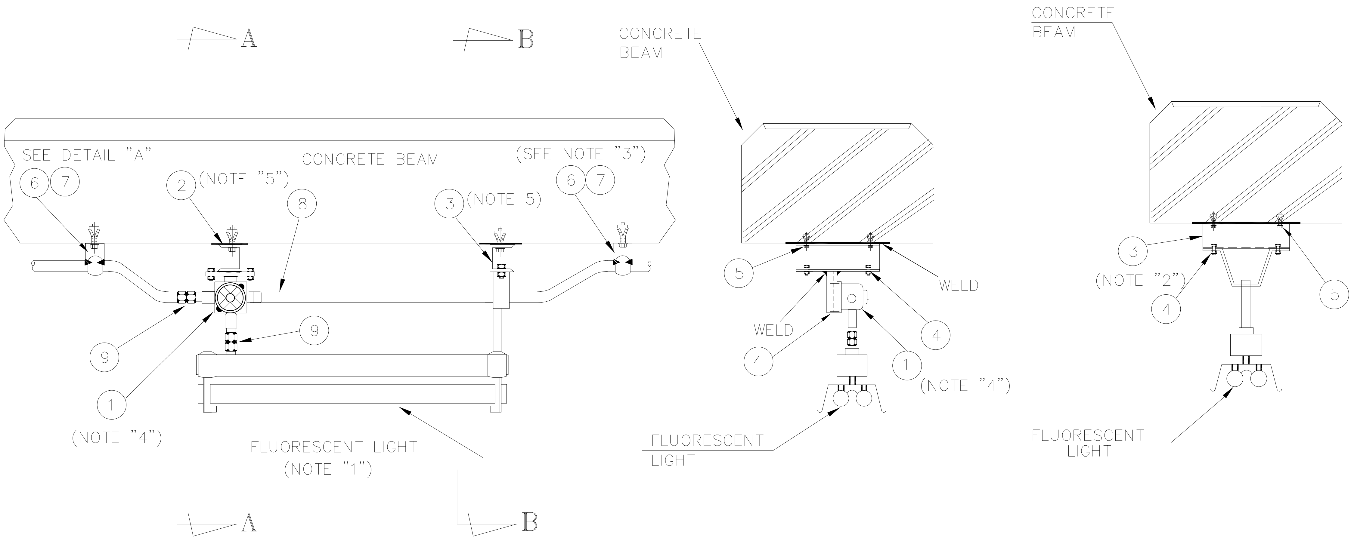
SECTION B-B
