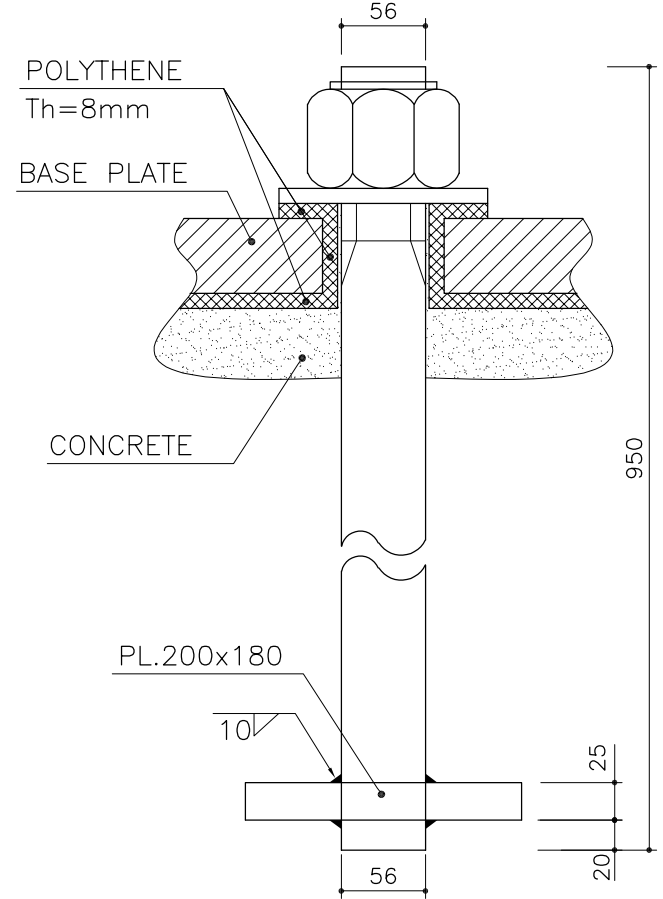
M56 HOT DIP GALVANIZED ANCHORBOLTS SC.1:5
