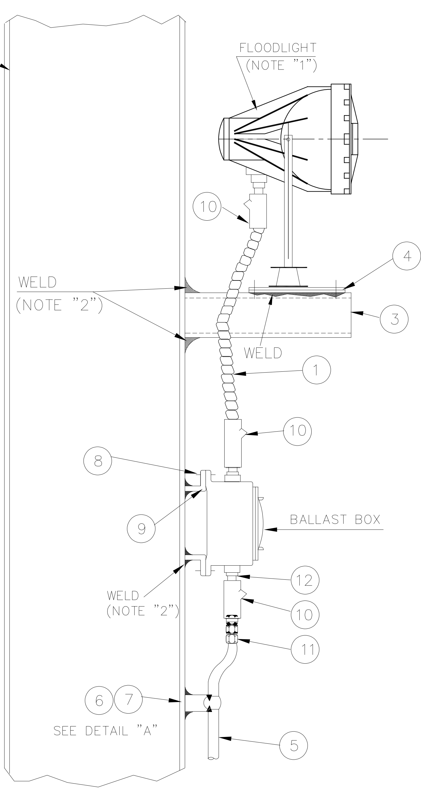
SIDE VIEW
