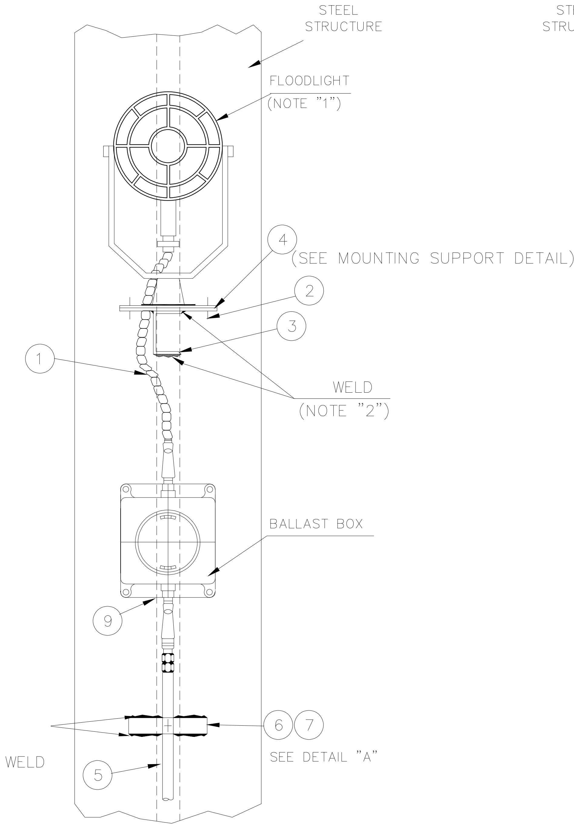
FRONT VIEW
