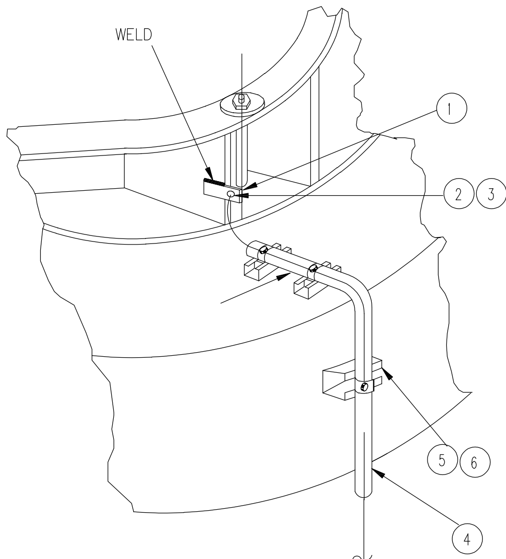
DETAIL "C"
