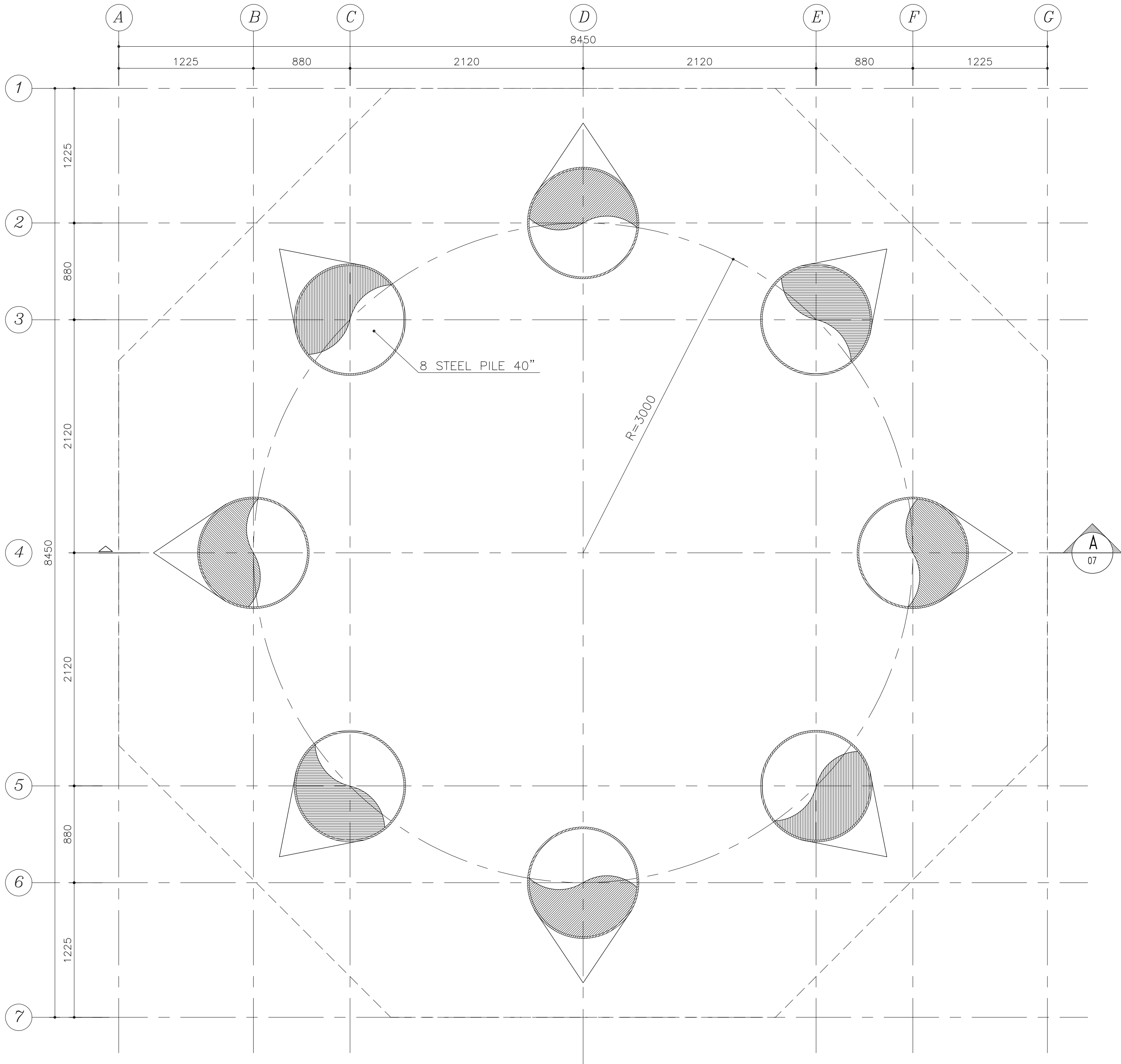
MOORING DOLPHIN PILING PLAN SC.1:25
