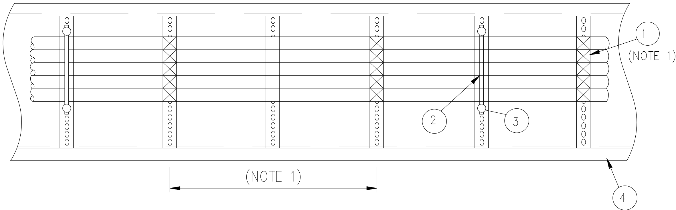
1) VERTICALLY TRAY MOUNTED. HORIZONTAL CABLE RUN
