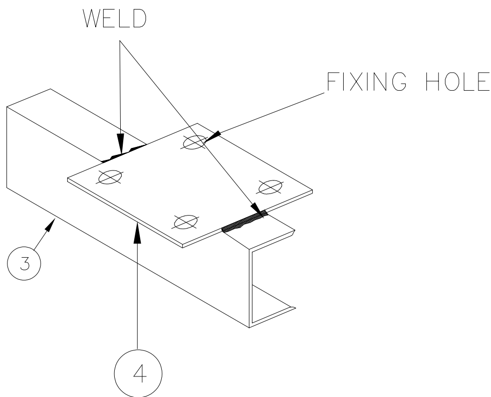
MOUNTING SUPPORT DETAIL
