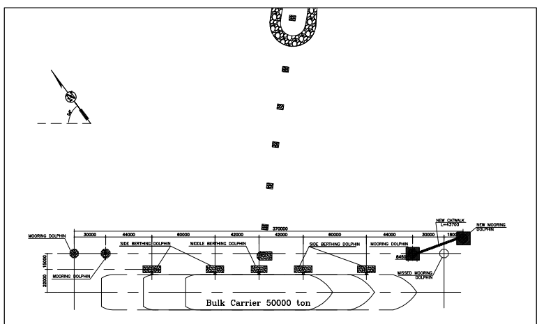
KEY PLAN
