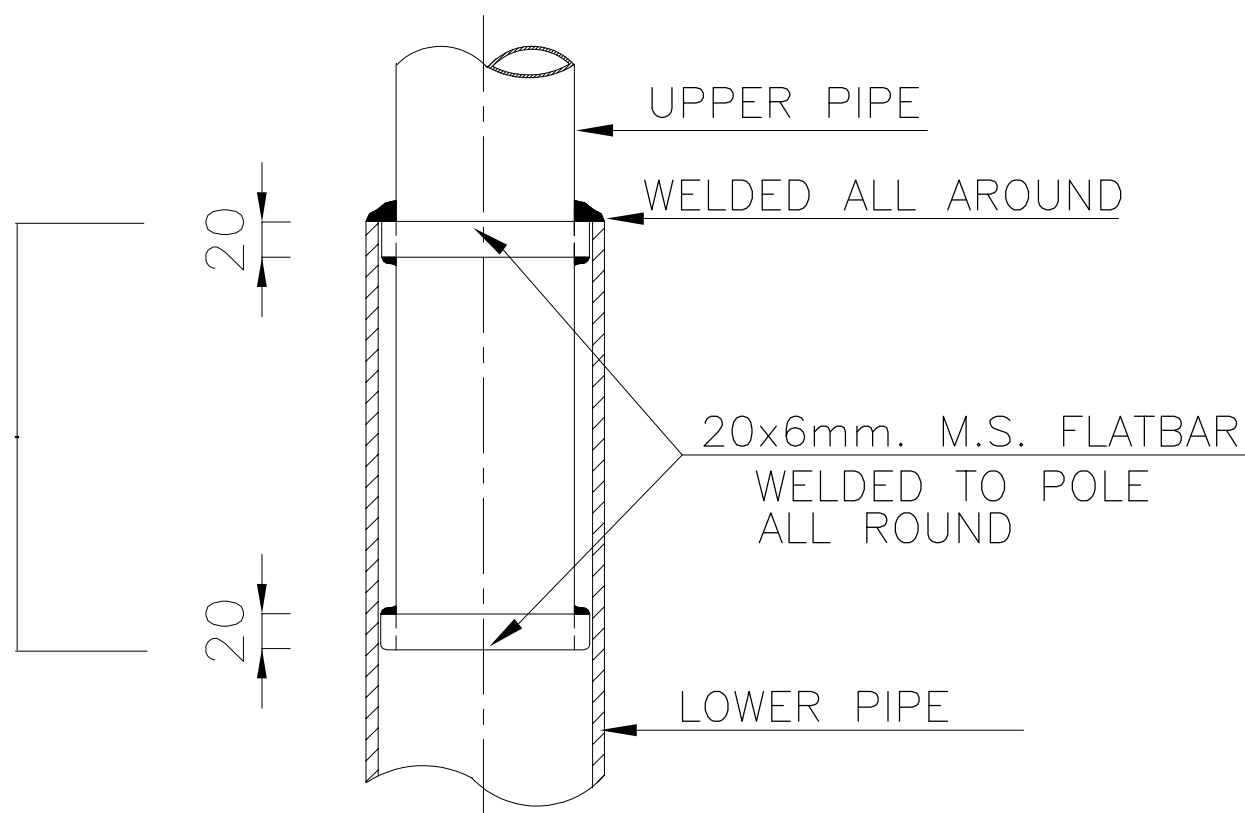
DETAIL "A" PIPE CONNECTION
