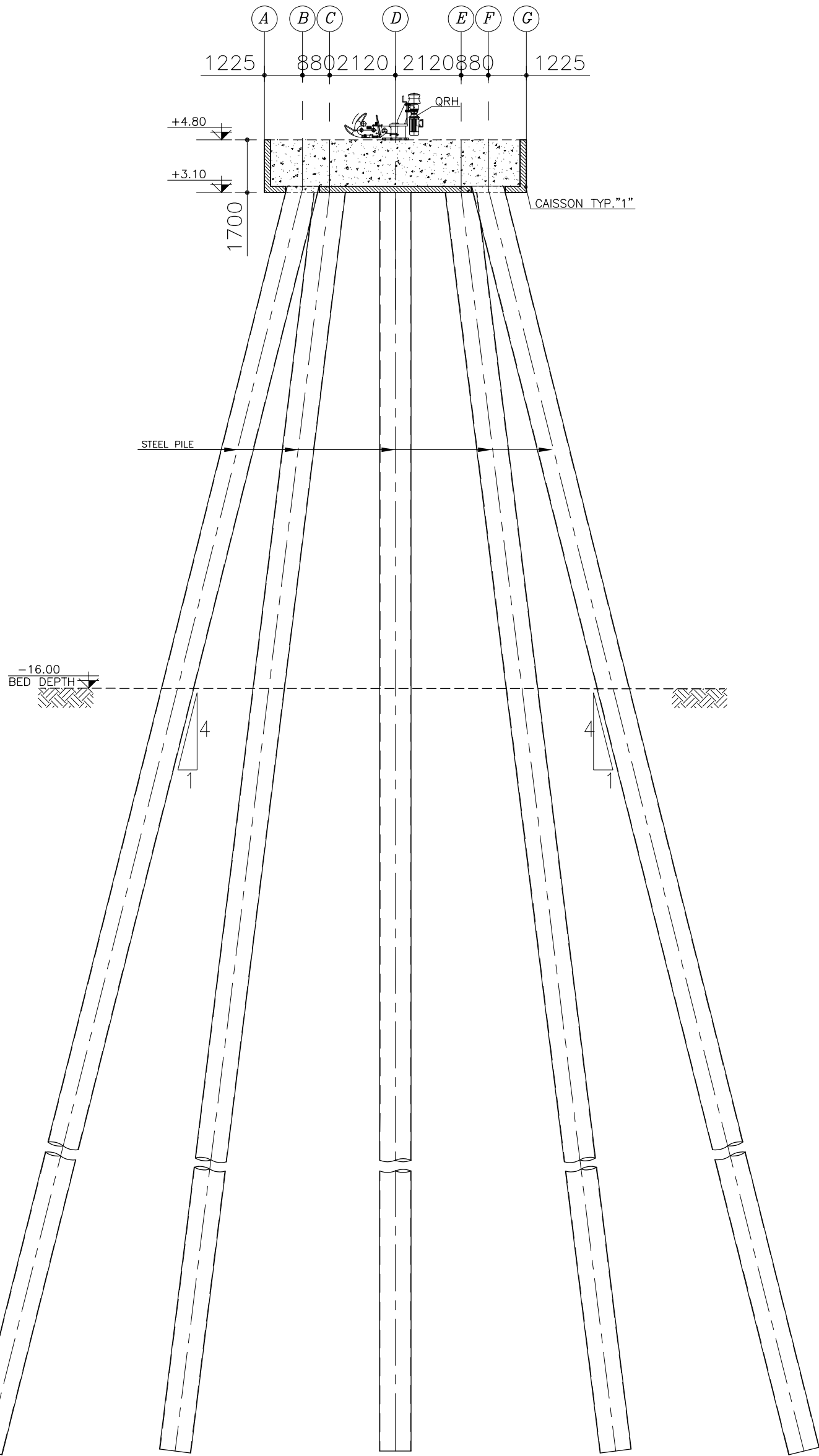
SECTION A SC.1:150
