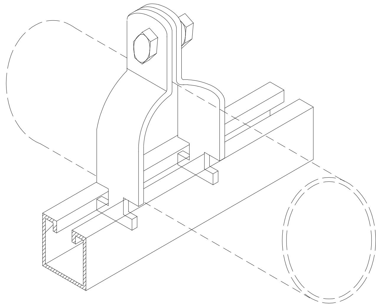
ISOMETRIC VIEW OF UNISTRUT CHANNEL & CLAMP
