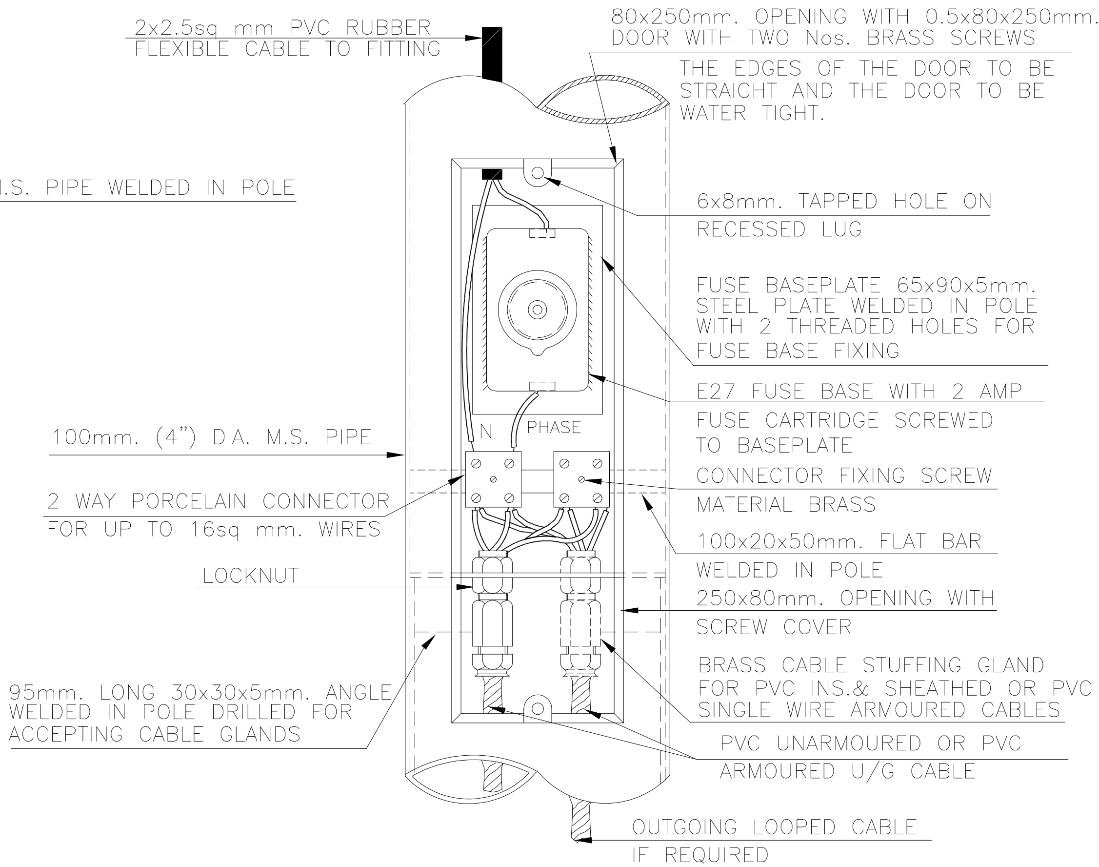
DETAIL "B" CABLE CONNECTION INSIDE THE POLE
