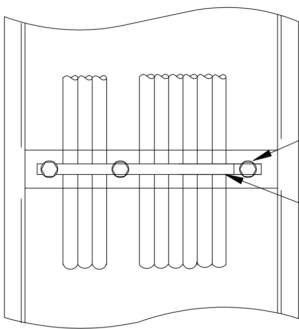
2) VERTICALLY TRAY MOUNTED. VERTICAL CABLE RUN
