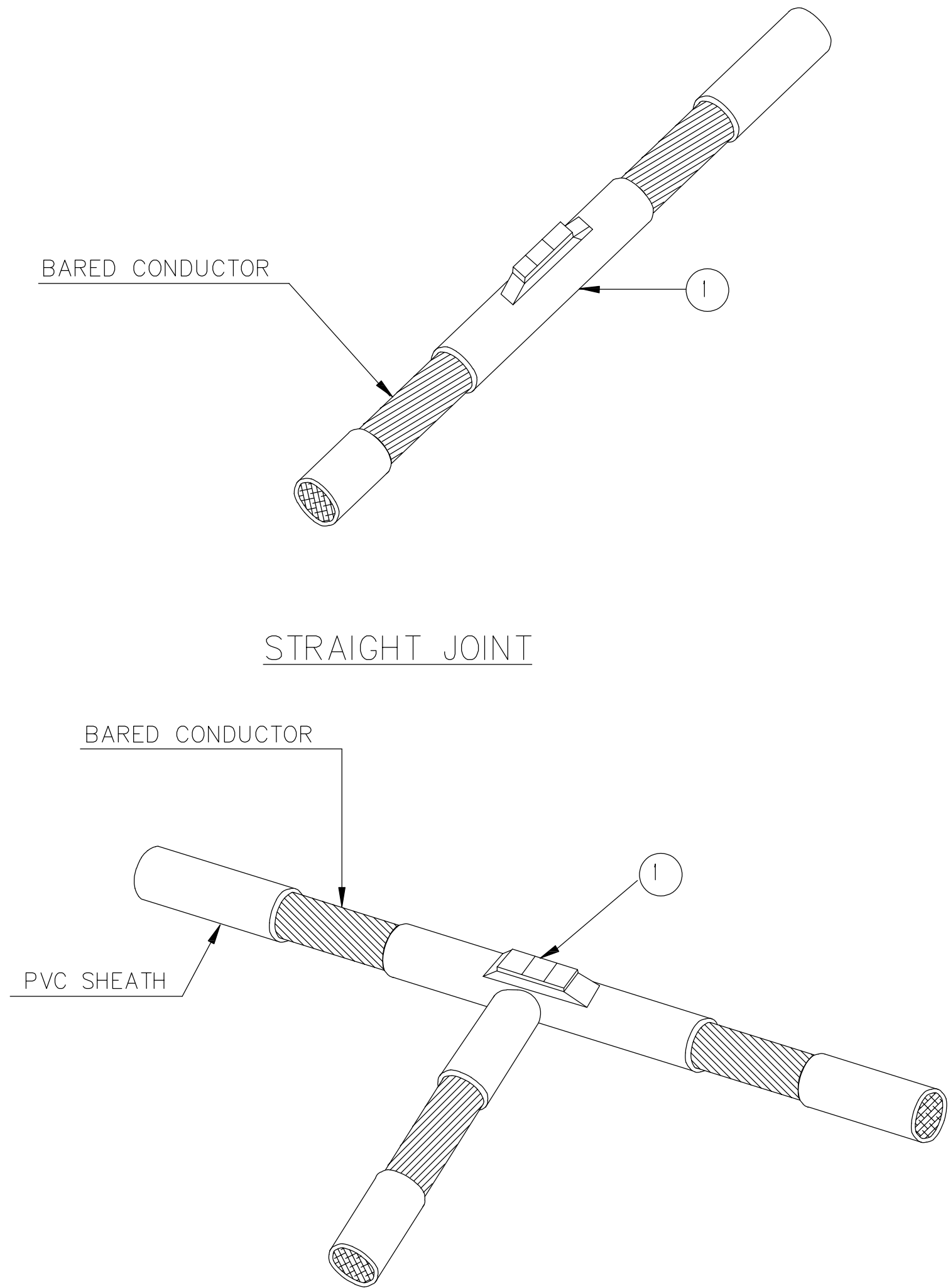
TEE BRANCH
