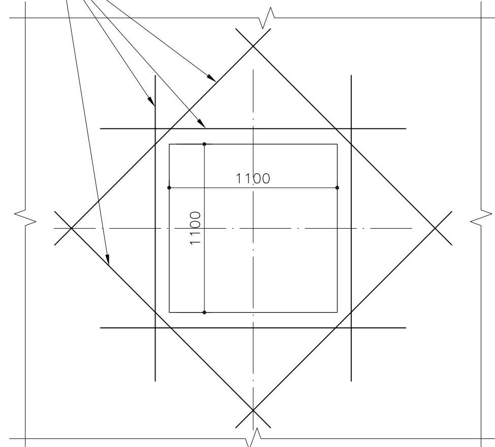
ADDBAR FOR OPENING SC.1:25
