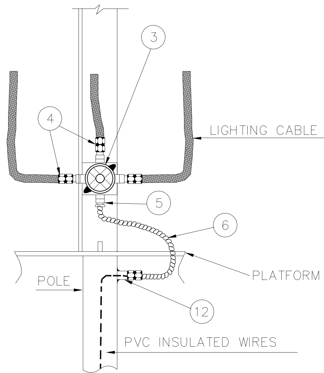
DETAIL "C"
