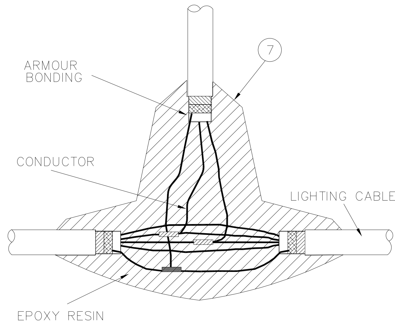
DETAIL "B"
