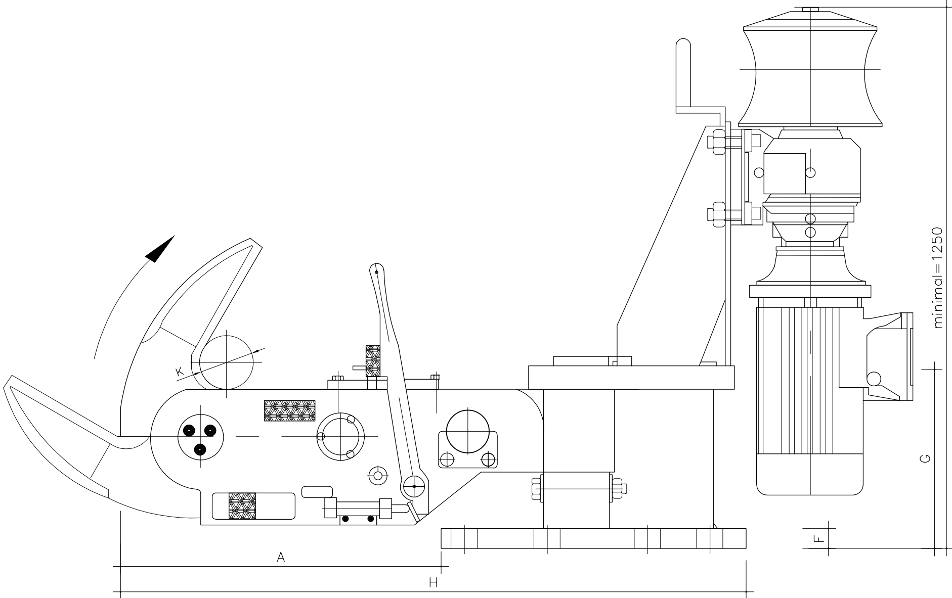
SECTION B 1:10
