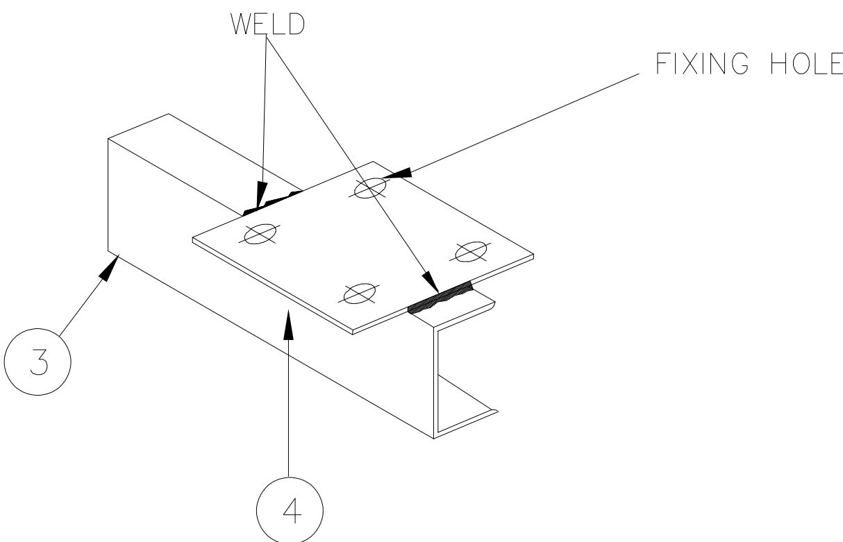
MOUNTING SUPPORT DETAIL
