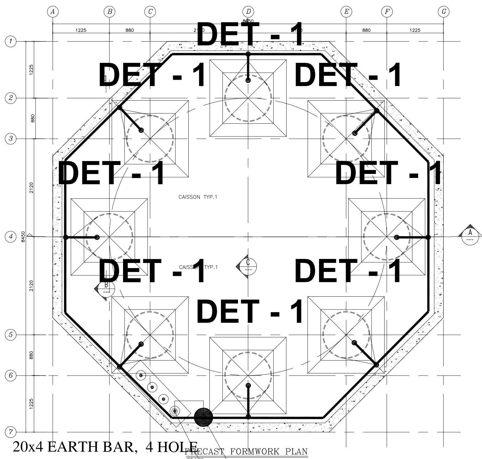
PRECAST FORMWORK PLAN
