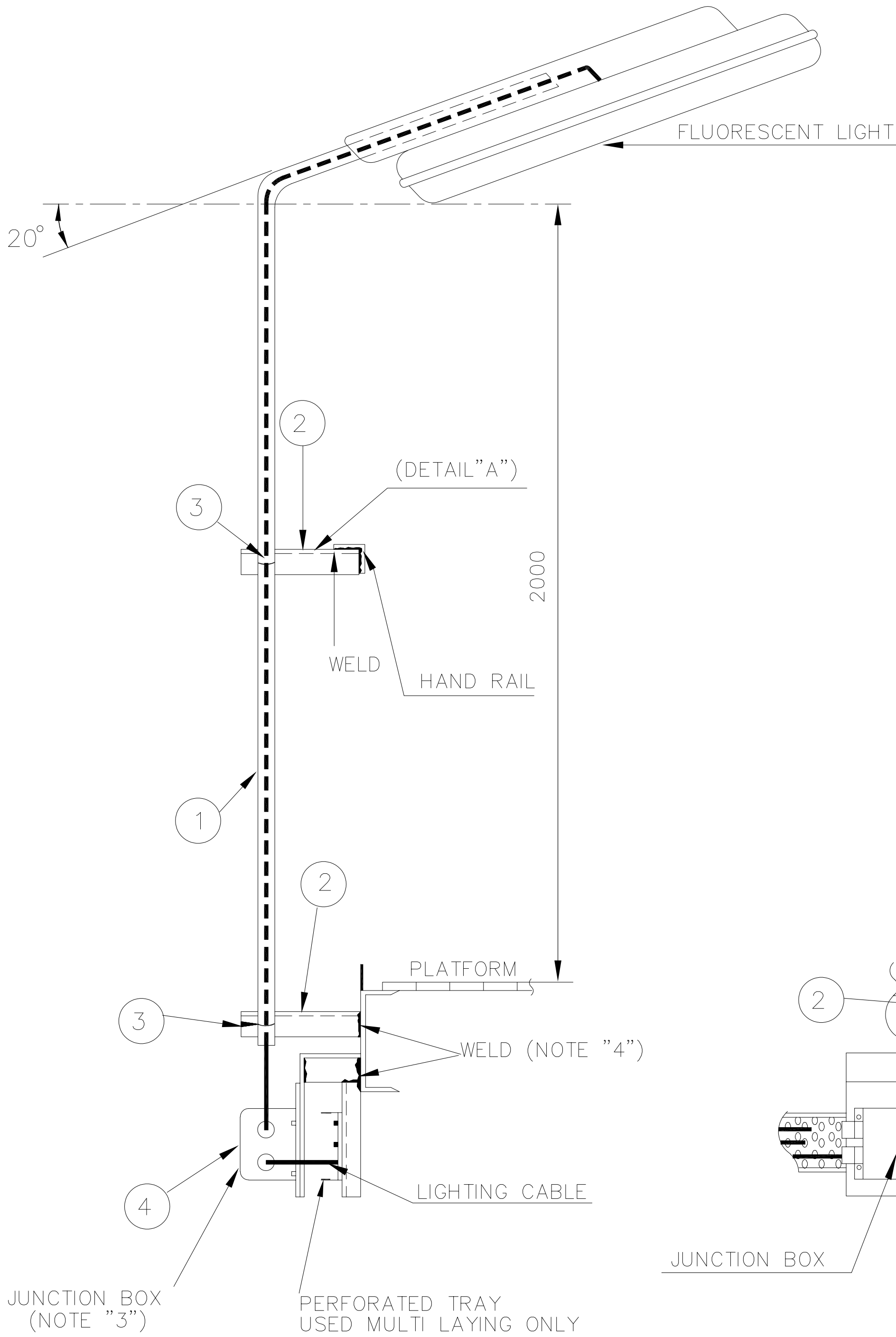
MULTI CABLE
