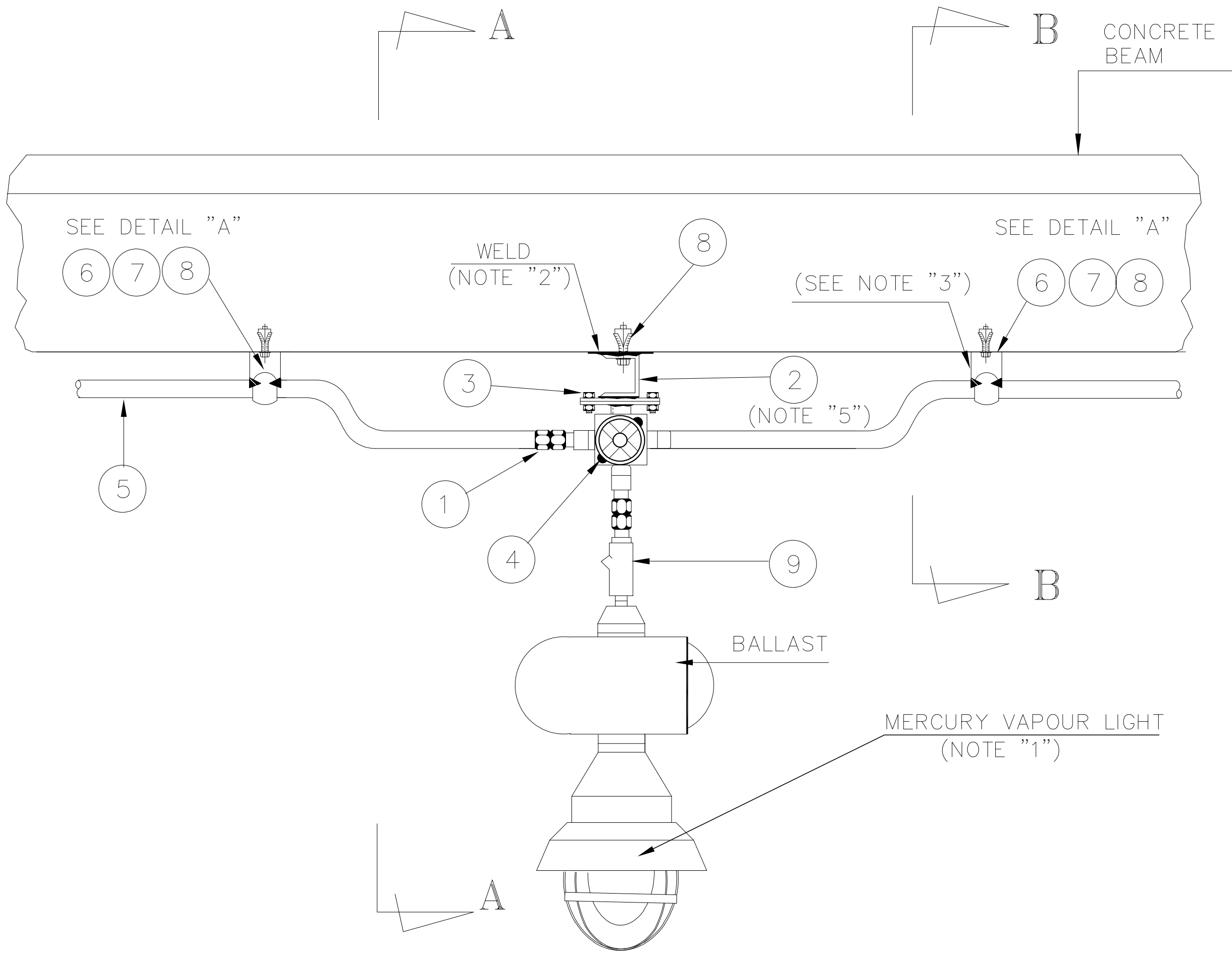
FRONT VIEW
