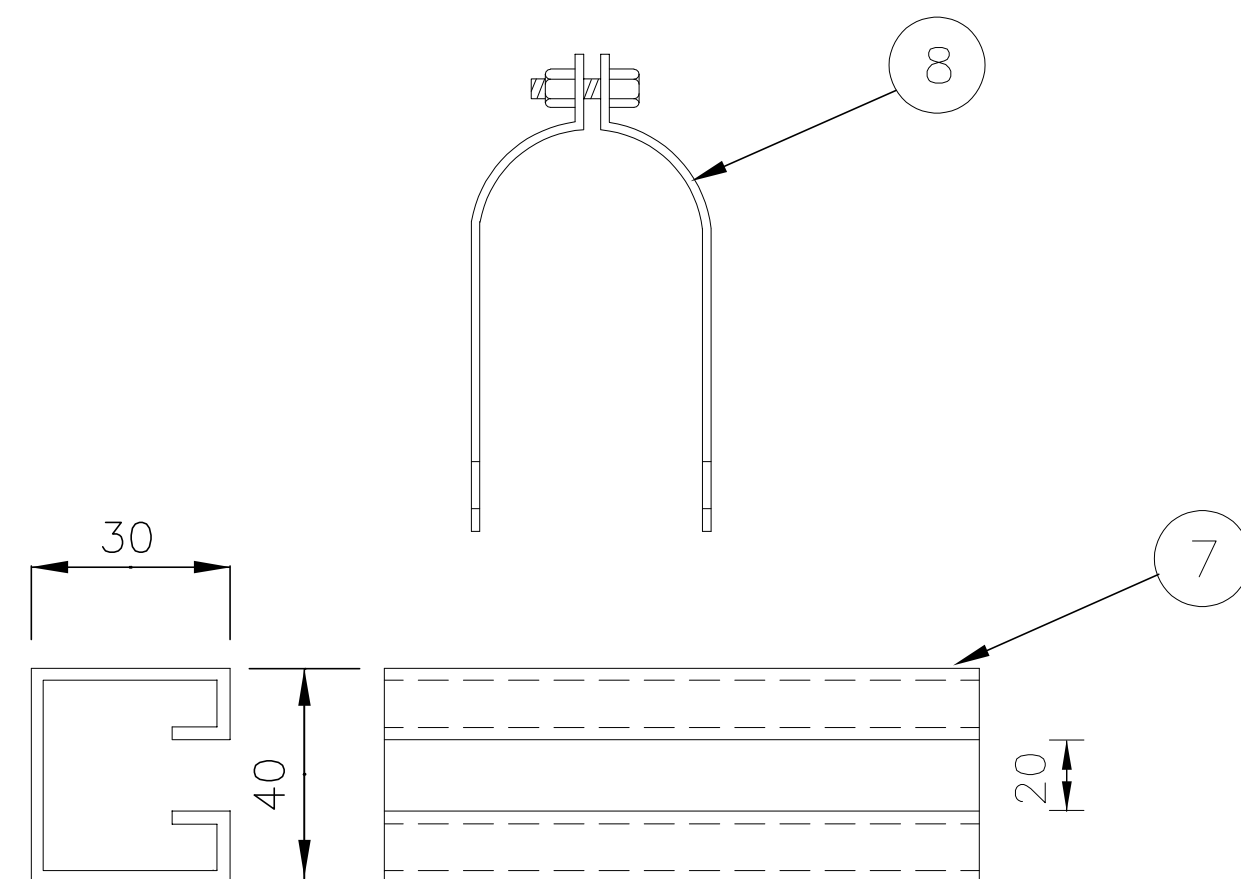
DETAIL "A"
